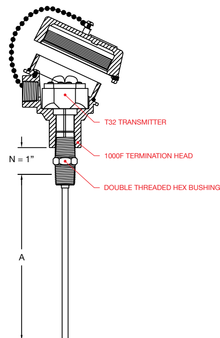
THERMOCOUPLE ASSEMBLY SAMPLE TC10-3-0-I-C-1AW13-6-DS-010-B-1-1-P-00600-Z
